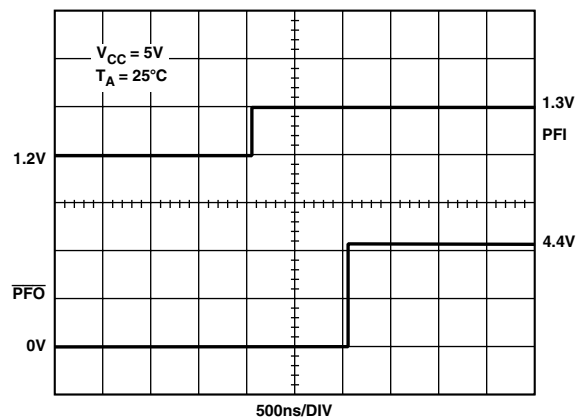
TPC 4. PFI Comparator Deassertion Response Time
