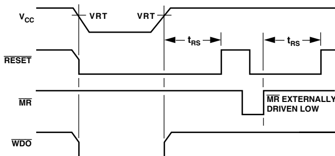
Figure 3. \overline{RESET} , \overline{MR} , and \overline{WDO} Timing
